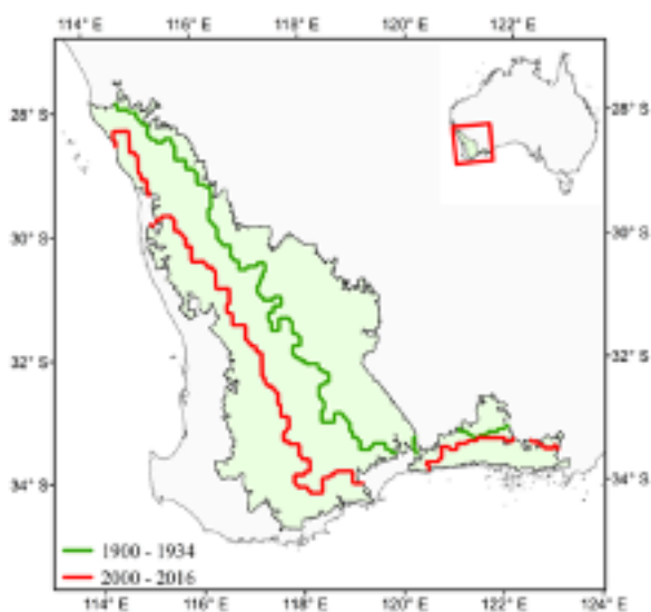
Figure 8. Shift in rainfall isohyets (left) and the 3t/ha potential yield line (right) over the past 100 years as the climate has dried across southwest Western Australia. Sources: left: DPIRD and right: Fletcher et al (2020) 5
